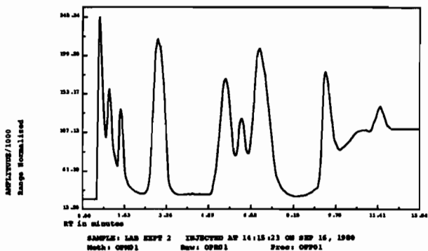
Figure 1. Raw chromatogram
