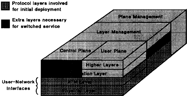
Figure 5. ATM layered architecture model.
