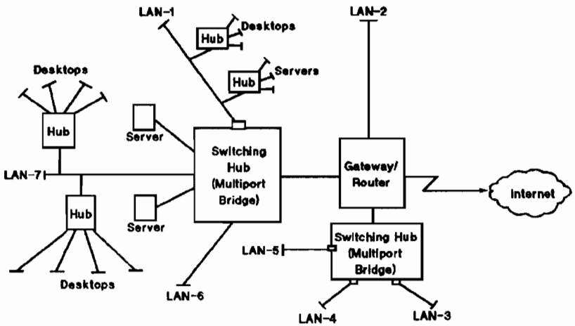
Figure 3. Multiple switching hubs incorporated in a LAN infrastructure can be configured to provide dedicated per port bandwidth for critical systems and applications.
