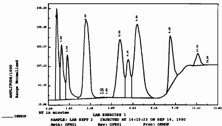
Figure 2. Processed chromatogram
